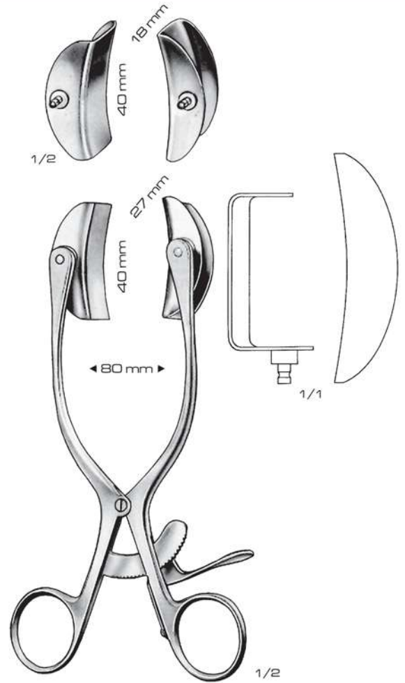
Baby-Collin 03-159-17 17 cm / 6 3/4" Abdominal retractor complete with 2 pairs of blades
